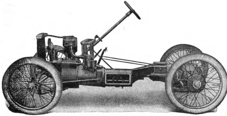
UNIQUE CHASSIS OF ROVER FRAMELESS ENGLISH LIGHT CAR.
